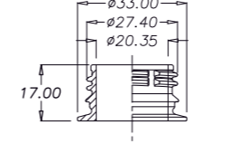
28mm PCO 1881 Thick Neck
