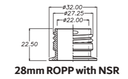
28mm ROPP with NSR
